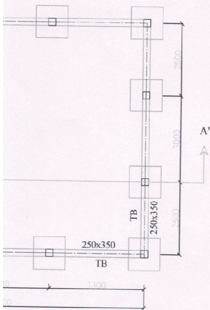
FOUNDATION LAYOUT OF ENCLOSURE
