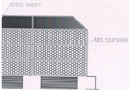
ELEVATION OF ENCLOSURE
