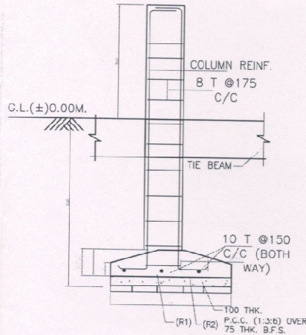
DETAIL OF SECTION 2-2 SCALE:1:50
