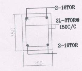
TYP. SEC OF TIE BEAM (TB) SCALE 1:30
