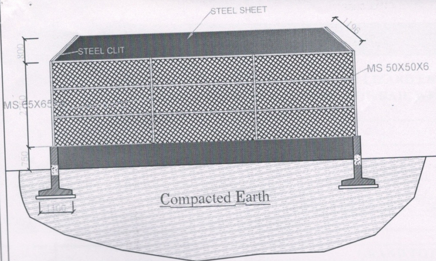
A-A' SECTION ELEVATION OF LIZARD ENCLOSURE
