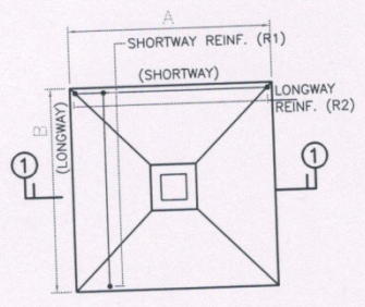
DETAIL OF FOOTING F3 SCALE-1:50
