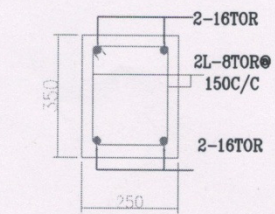
TYP. SEC OF TIE BEAM (TB) SCALE 1:30
